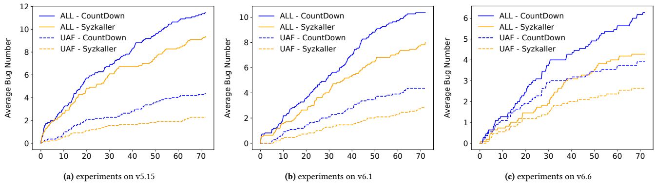
Figure 8: Bugs detected by COUNTDOWN and SYZKALLER on three kernel versions. All numbers are average from 11 runs of 72-hour experiments. All the comparisons are statistically significant (p-values < 0.05).
