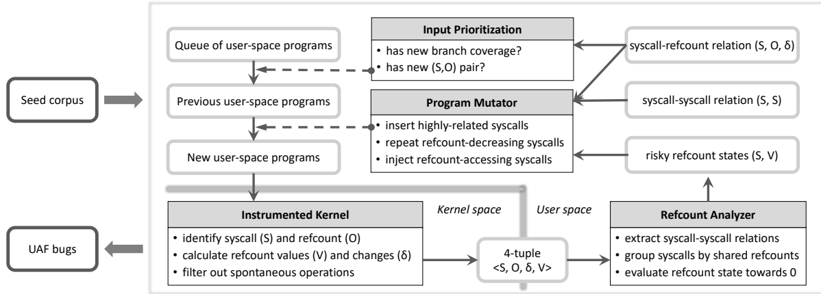
Figure 6: Overview of COUNTDOWN. Given a set of user-space programs, we will collect kernel execution traces to understand how each syscall updates refcounts. We use this information to build a new relation between syscalls and use the new relation to guide input prioritization and mutation.
