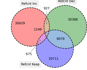
Figure 15: Refcount operations triggered in Linux v6.6 update refcount unidimensionally usually.
