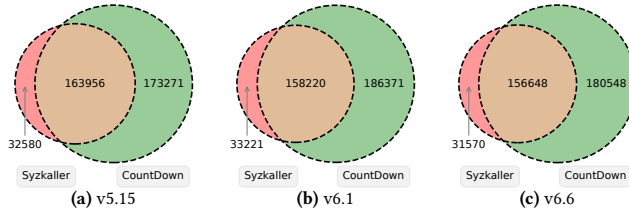
Figure 13: Relations learned by COUNTDOWN and SYZKALLER on three kernel versions. COUNTDOWN learns more unique relations than SYZKALLER and more than 80% relations learned by SYZKALLER are learned by COUNTDOWN.
